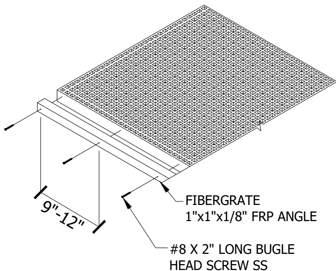
ISOMETRIC VIEW
