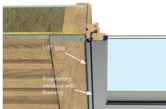
Fig. 26 - Window jamb with Enhanced Grain
