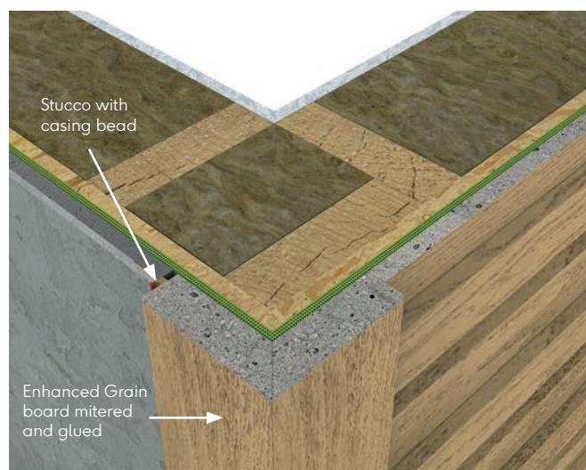
Fig. 30 - Corner detail to stucco
