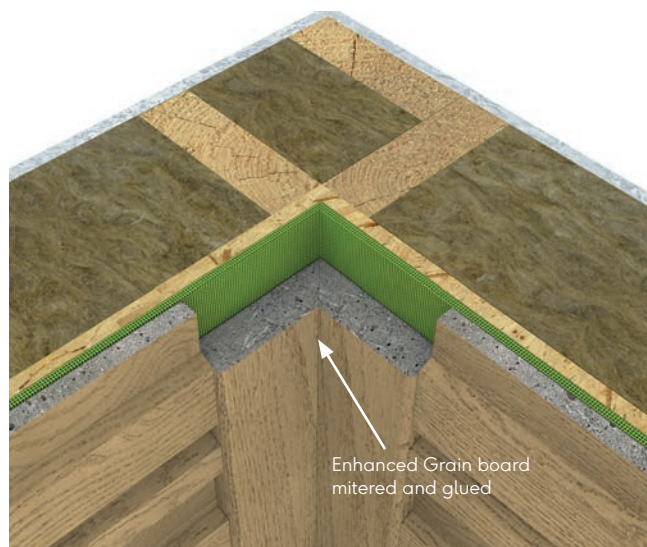
Fig. 12 - Mitered corner board detail
