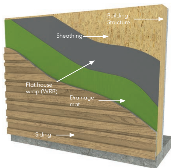
Fig.3 - Typical wall build-up with rainscreen drainage mat
