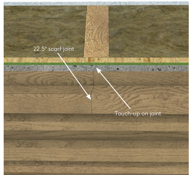
Fig.21 - Board joint
