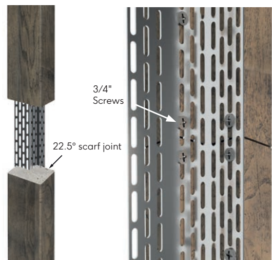
Fig. 11 - Joining corner profiles
