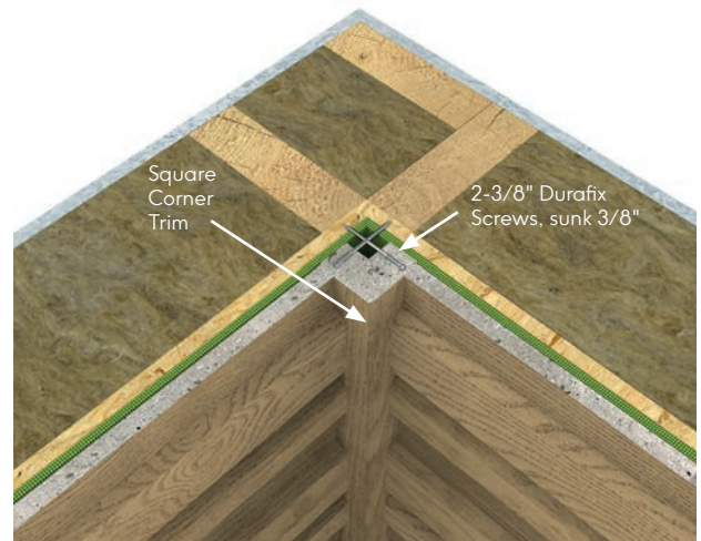
Fig. 9 - Internal corner profile
