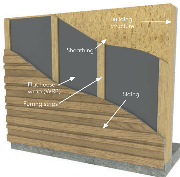
Fig.4 - Typical wall build-up with furring strips
