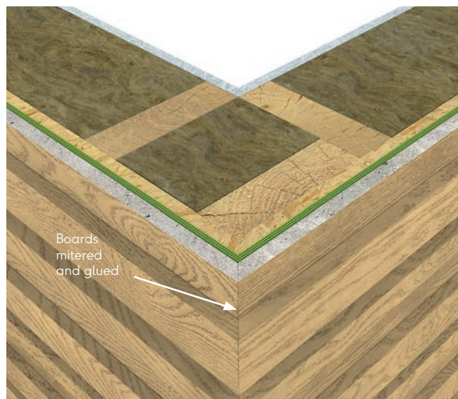
Fig. 13 - External corner Miter detail
