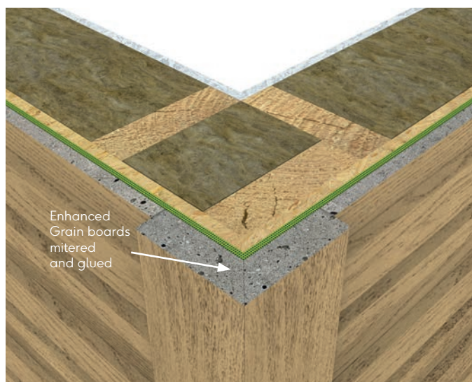
Fig. 15 - Mitered Corner board detail
