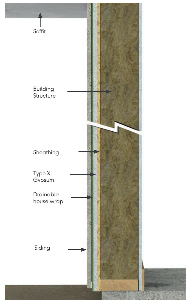
Fig.1 - Typical construction for WUI zones
