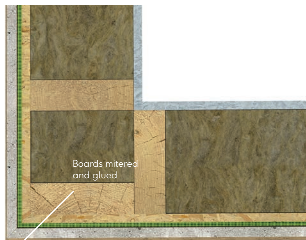
Fig. 13 - External corner Miter detail
