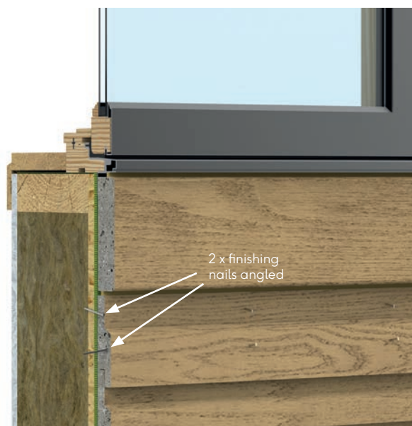
Fig.20 - Typical finishing nail detail - Window sill
