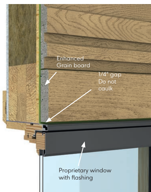
Fig. 25 - Window head with Enhanced Grain
