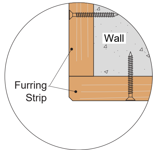
Detail 18-5
