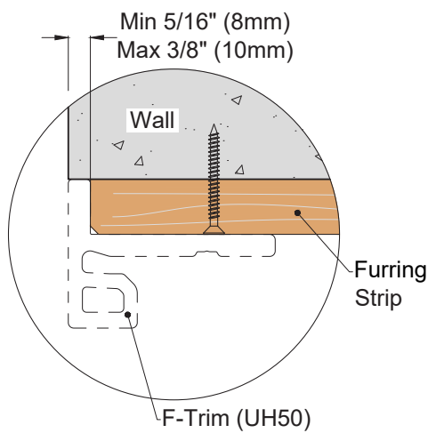
Detail 18-3
