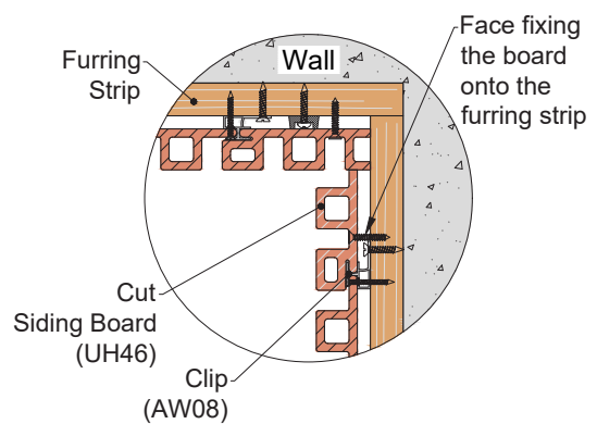
Detail 26-5
