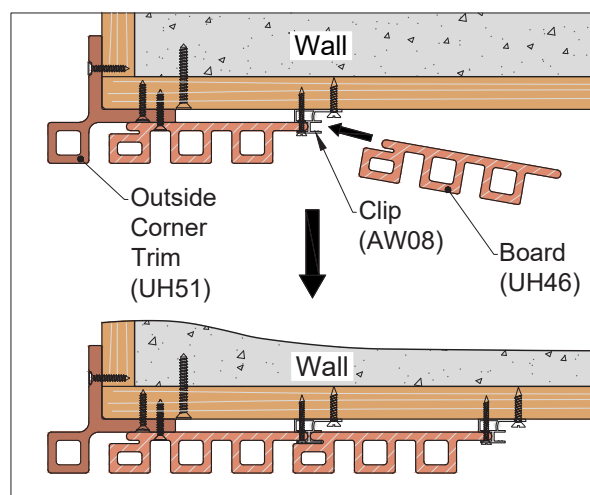
Detail 22-4
