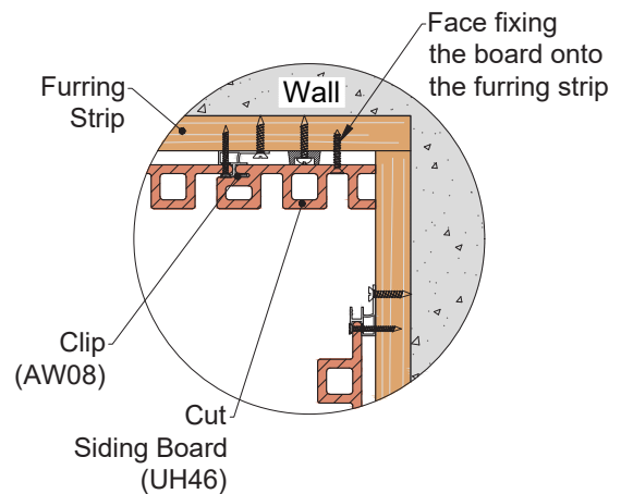
Detail 26-4
