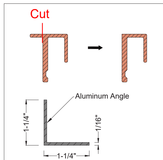
Detail 27-2-1
