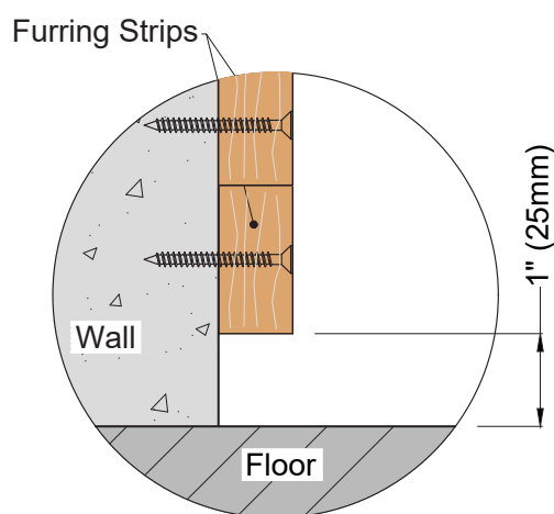
Detail 18-1
