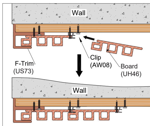
Detail 22-2
