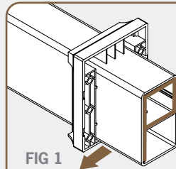
FIG 1 Long leg of P-Shaped Aluminum Stiffener needs to face towards inside of deck.
