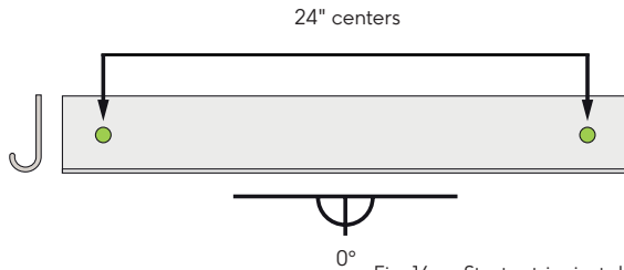
Fig. 16a - Starter trim install
