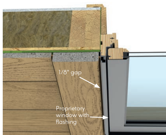
Fig. 26 - Window jamb with Enhanced Grain
