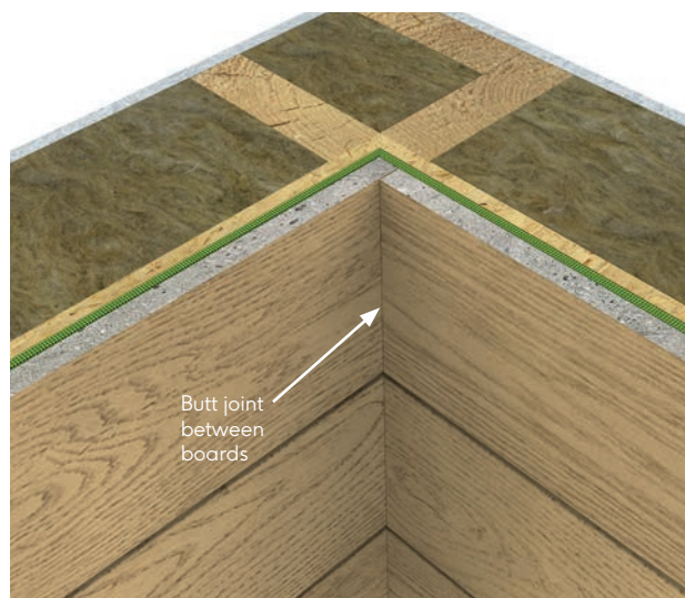
Fig. 12 - Internal corner butt joint
