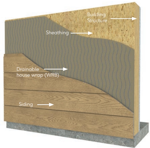
Fig.2 - Typical wall build-up with drainable housewrap
