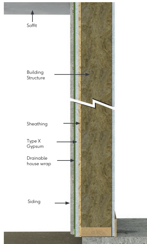
Fig.1 - Typical construction for WUI zones
