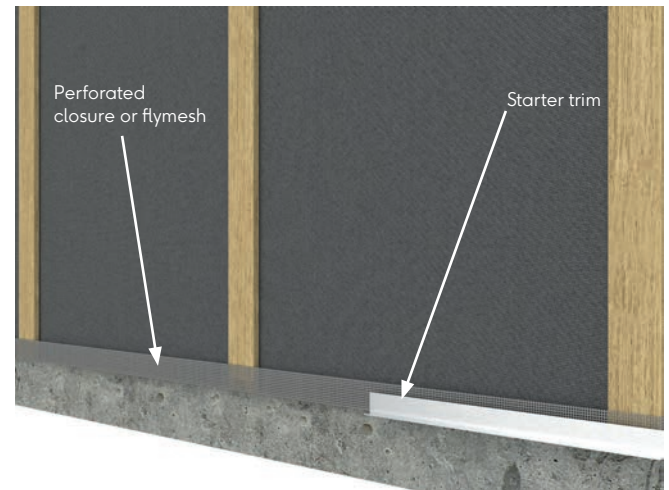
Fig.5 - Insect invasion prevention
