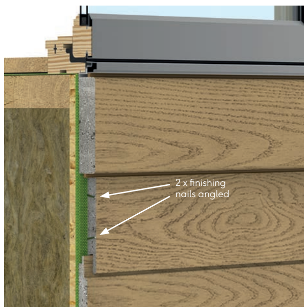
Fig.20 - Typical finishing nail detail - Window sill
