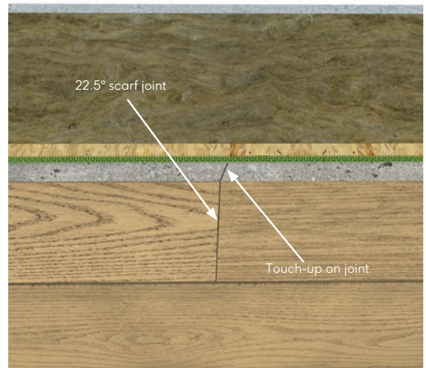
Fig.21 - Board joint
