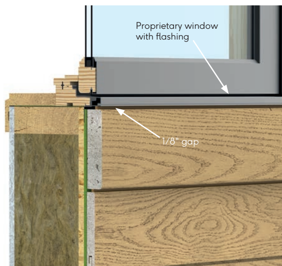
Fig. 27 - Window sill with Enhanced Grain
