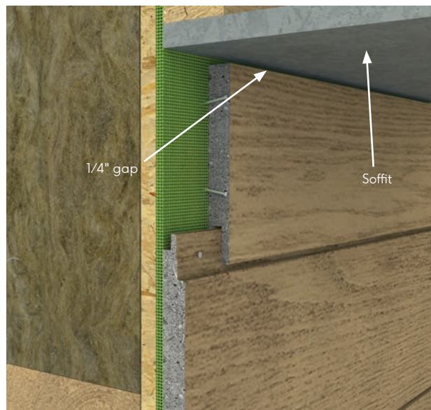
Fig. 19 - Wall head
