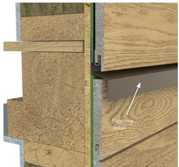
Fig.22 - Horizontal joint
