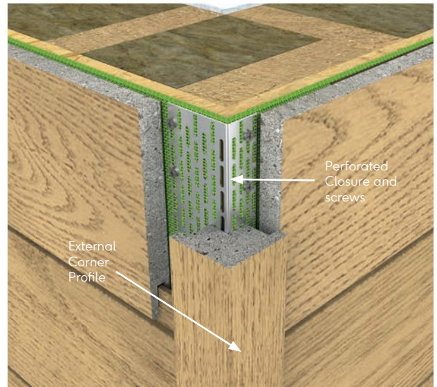
Fig. 10 - External corner profile
