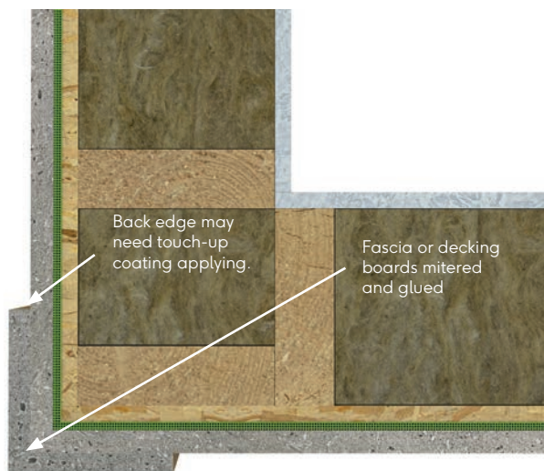
Fig. 14 - Mitered corner top view
