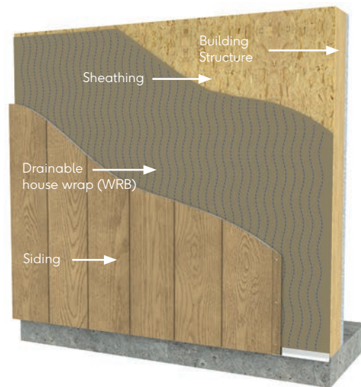
Fig.2 - Typical wall build-up with drainable housewrap
