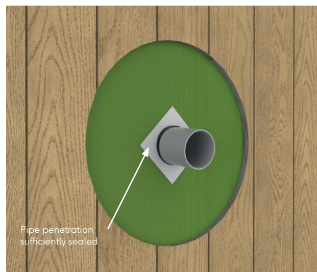
Fig.30 - Wall penetration
