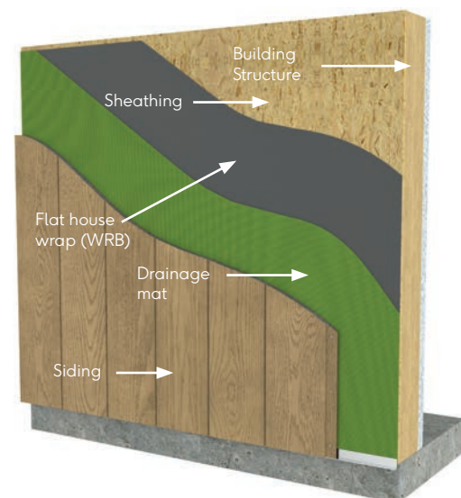
Fig.3 - Typical wall build-up with rainscreen drainage mat
