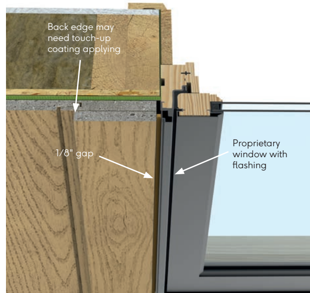
Fig.29 - Window jamb with fascia boards
