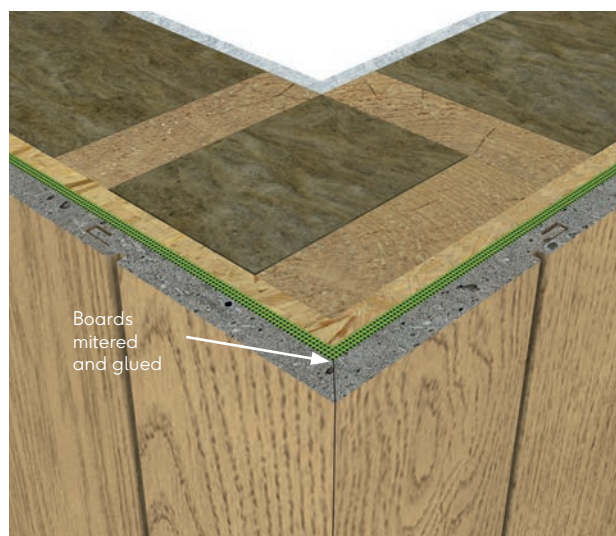
Fig. 13 - External corner miter joint
