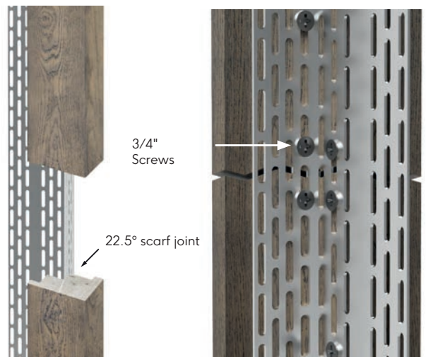
Fig. 11 - Joining corner profiles
