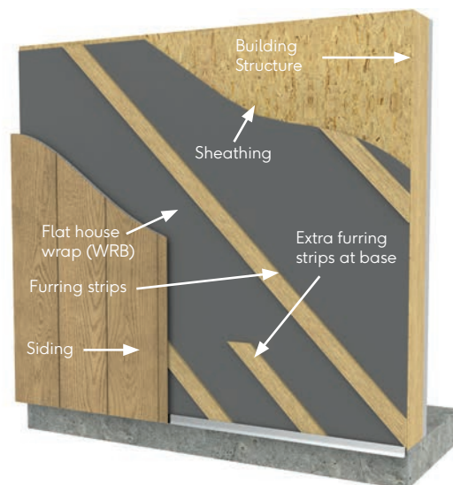
Fig.4 - Typical wall build-up with furring strips
