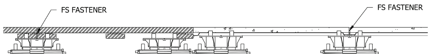
AS SHOWN: BISON WOOD PAVER WITH 2CM PAVER AND BISON PAVER TRAY
