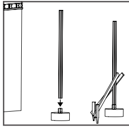
2. Mount Posts To Footing and Brace
